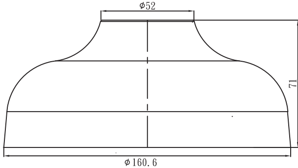
NDA-4020-PIP Pendant interface plate Dimensions in mm (inch)
